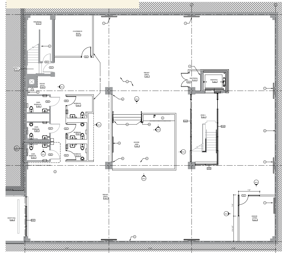
LOWER LEVEL FLOOR PLAN
